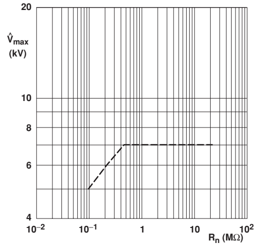
Maximum allowed peak pulse voltage in accordance with "IEC 60065 chapter 14.1"; 50 discharges from a 1 nF capacitor charged to V max ; 12 discharges/minute (drift ΔR/R ≤ 2 %).
