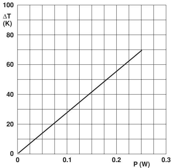
Hot-spot temperature rise (ΔT) as a function of dissipated power.
